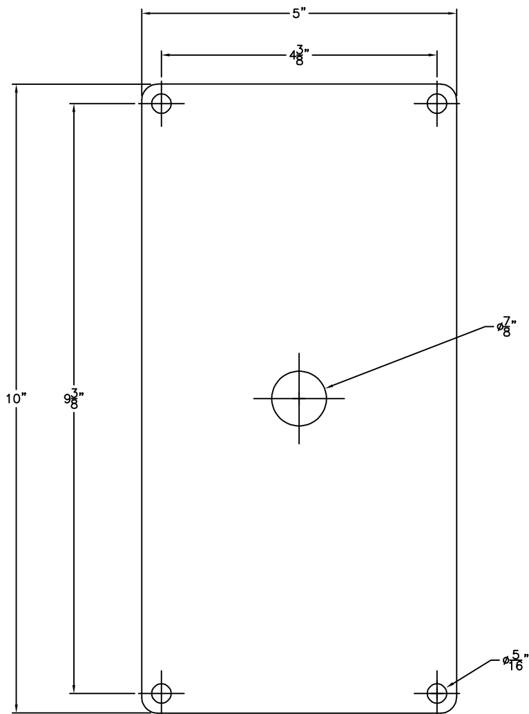
MOUNTING HOLE DIMENSIONS (NOT TO SCALE)
